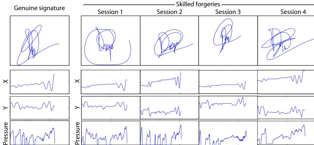
Figure 4. Signature examples from the BiosecurID Database. The left sample is a genuine signature and the remaining ones are forgeries with incremental level of skill. In each case, plots below each signature correspond to the on-line information stored in the database.
