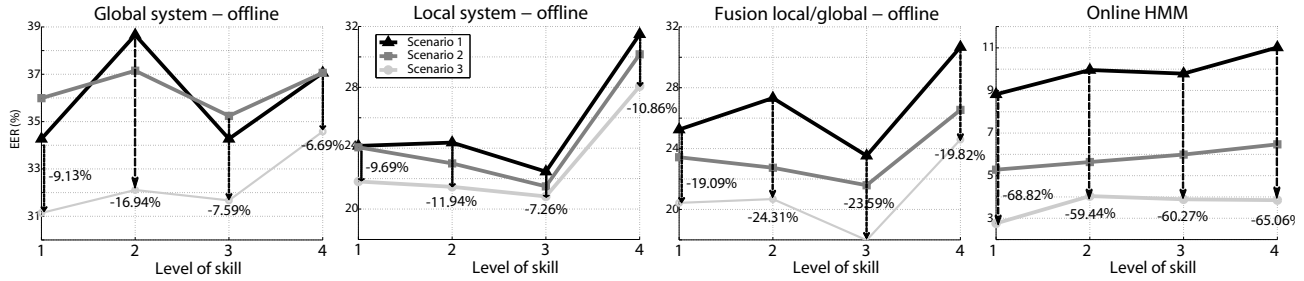
Figure 6. Verification performance based on the level of skill in the forgeries for the different scenarios presented in Section 4.2. Results are given in terms of Equal Error Rates (in %). For each level of skill, it is also given the relative gain of performance of the scenario 3 with respect to the scenario 1.
