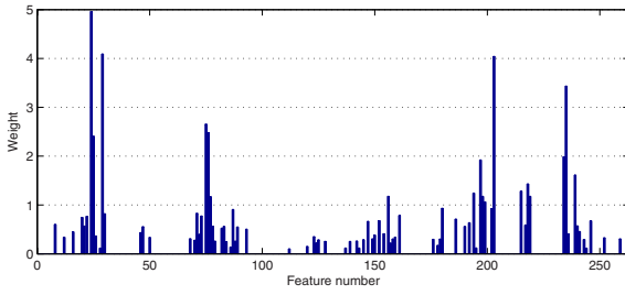
Fig. 5. Addition of all the weights assigned by all the trained AdaBoost classifiers for each feature
