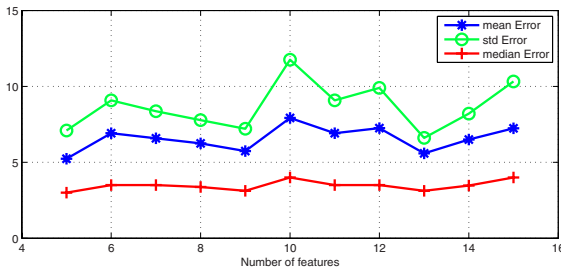
Fig. 6. Evolution of the mean error (in blue, stars), standard deviation (in green, circles) and the median of the error (in red, crosses) of each multiple classifier
