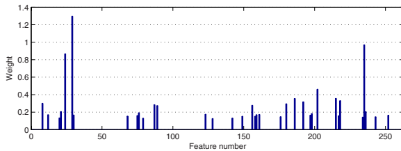
Fig. 4. Selected features by one AdaBoost classifier and their weights
