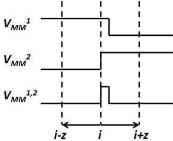
Figure 1. Interruption measurement.
