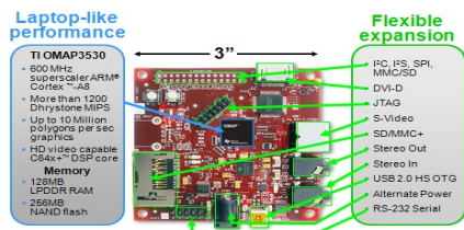
Figure 3: Beagleboard front view, from [3].
