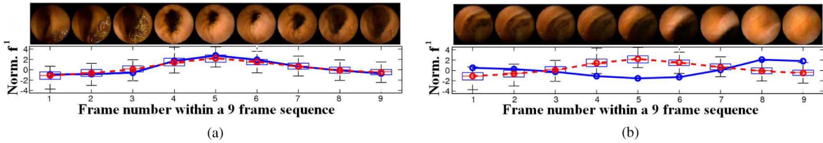
Fig. 5. Pattern of f^1 (solid blue line) for (a) one contraction and (b) a random sequence. The dashed red line corresponds to the averaged pattern of all the labeled intestinal contractions and the box plots define their lower quartile, median, and upper quartile (the whiskers show the extent of the rest of the data).
