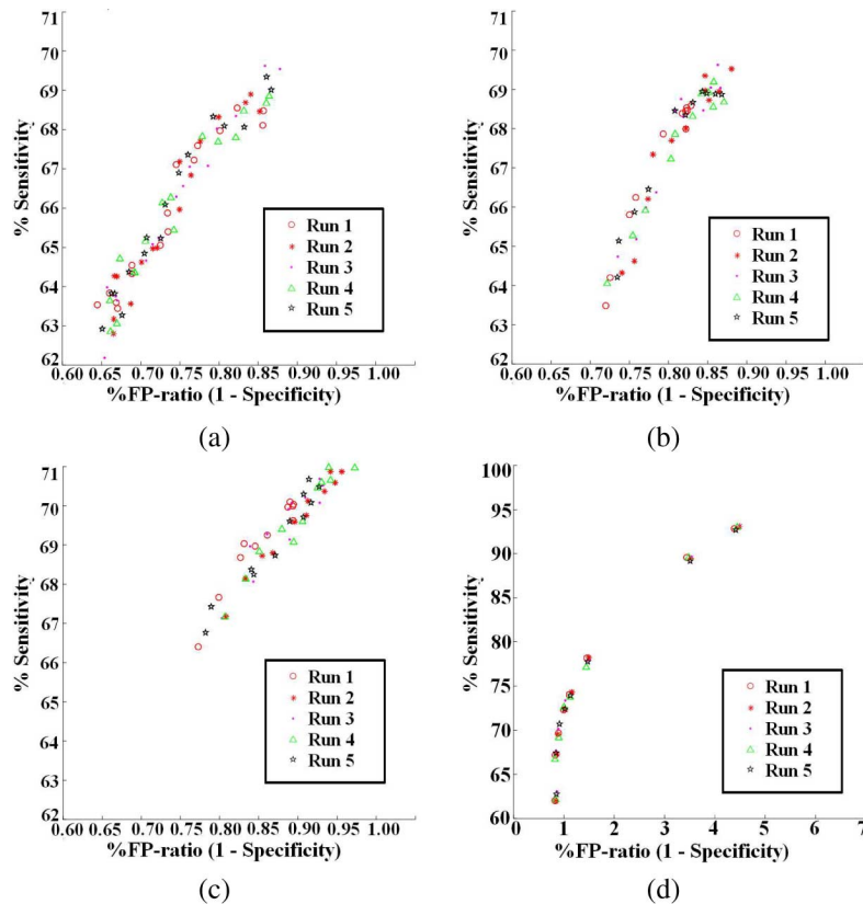
Fig. 12. Operation points from the ROC curve segments using the forward parameter selection procedure for (a) P_1 , (b) P_2 , (c) P_3 , and (d) P_4 . Each symbol represents each of the different five runs. The different points of each symbol represent the different performance pairs of sensitivity versus FP-ratio.
