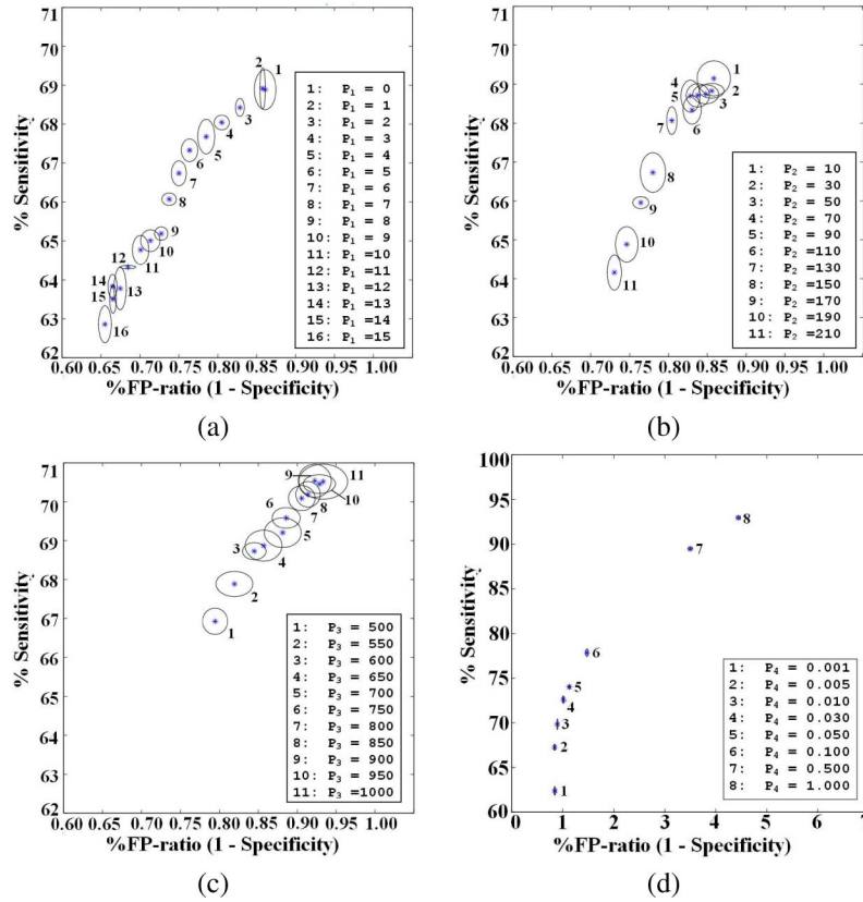
Fig. 13. Operation points from the ROC curve segments using the forward parameter selection procedure for (a) P_1 , (b) P_2 , (c) P_3 , and (d) P_4 , grouped by parameter value. The mean of each ellipse represents the mean of the performance pair obtained for that parameter after five runs. The axes of the ellipses are proportional to the resulting mean variance.
