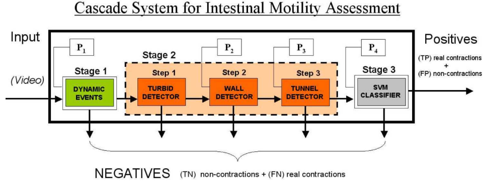
Fig. 4. Cascade system for intestinal motility assessment. The input is the video study and the output are the intestinal contraction frames suggested by the system. Each stage rejects sequences of noncontractions. The global performance can be tuned by the set of parameters P .
