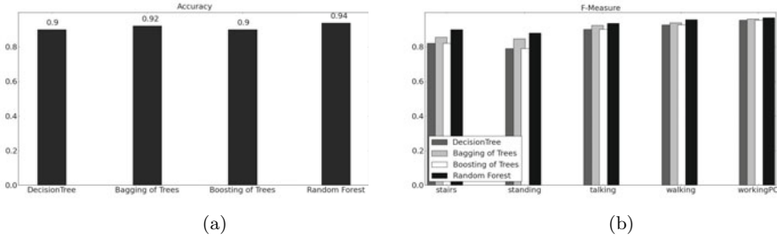
Fig. 3. (a) Classification Accuracy for Different Classifiers. (b) F-Measure for each Activity on the Motion Dataset.
