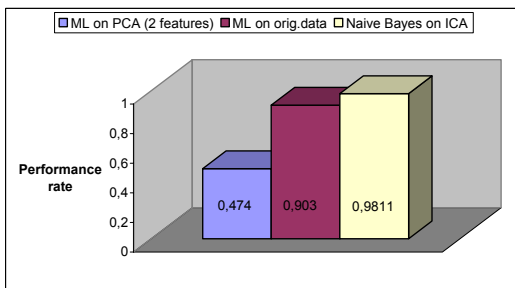
Fig. 6 Results of parametric classification
