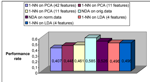
Fig. 5 Dependence on data representation.
