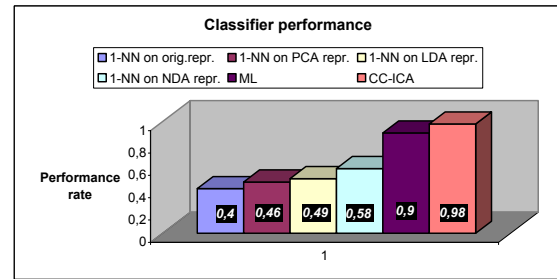
Fig. 3 Classifier Performance.
