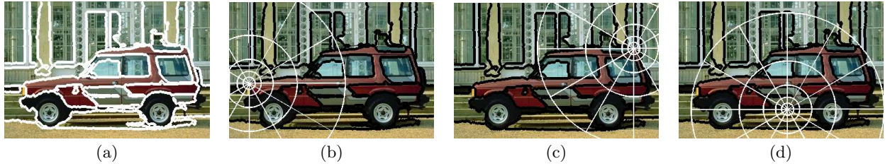
Figure 1: (a) Dense cloud of points covering interesting parts of the image (edges). (b)-(d) Three contextual descriptors using log-polar spatial quantization. Each descriptor represents a different ‘‘point of view’’ of the object’s spatial arrangement.
