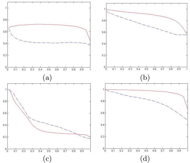
Figure 6: Precision-recall in Fergus database. The discontinuous line represents results obtained with our contextual descriptor and the continuous line with the shape context. See text.
