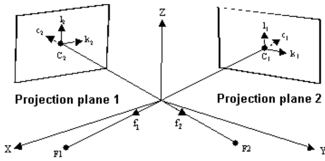
Figure 11. Global reference system (x,y,z) with the projection planes and their local systems.
