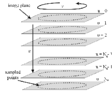
Figure 4. Two-dimensional B-Spline model space generalization.
